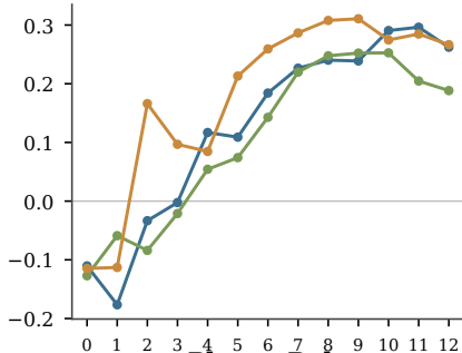
Phrase Role
