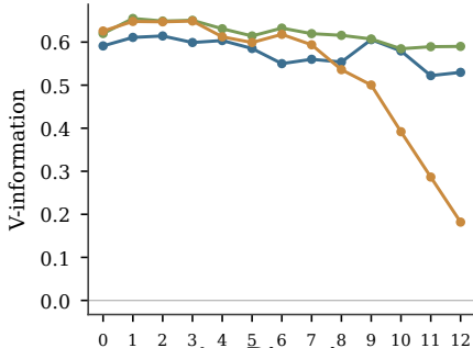
Arc Direction
